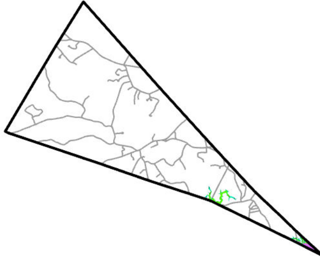
SLR + SS
