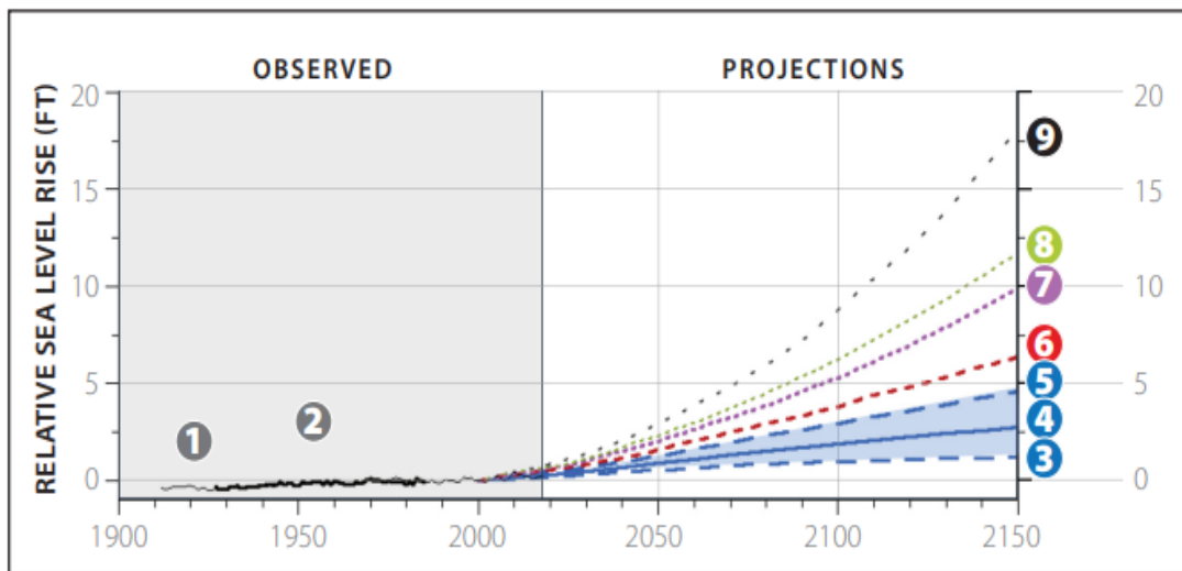
Figure 4.5. Observed and Projected Relative Sea-Level Rise for Seavey Island Tide Gauge K14 Projections | Stabilized Greenhouse Gas Concentrations (RCP 4.5).
